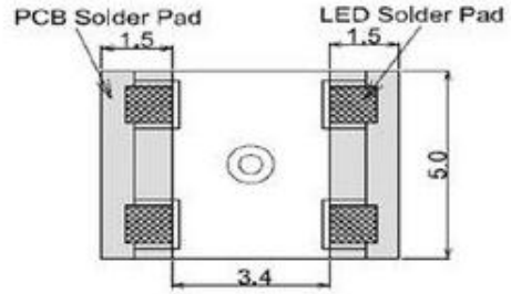
建议焊盘尺寸图 Recommended Soldering Pattern
